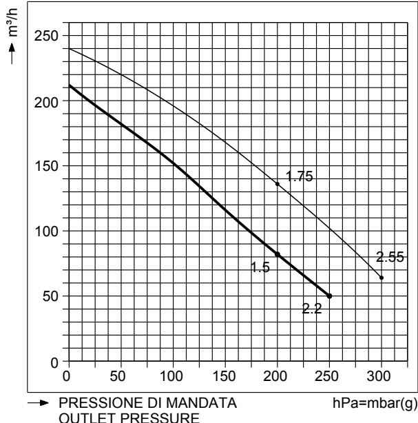
Prestazioni a 50Hz (2900giri/min.) - Performance at 50Hz (2900rpm) Prestazioni a 60Hz (3500giri/min.) - Performance at 60Hz (3500rpm)
